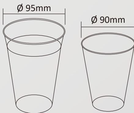
Standard mold for 95 mm PP cups and 90mm paper cups.
